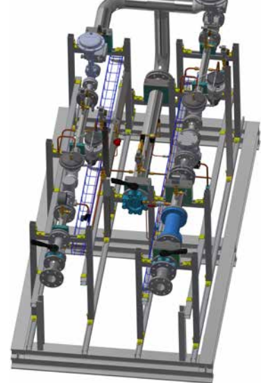
SNG mixer
