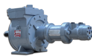
Pump type FAS-Corken with hydraulic motor
